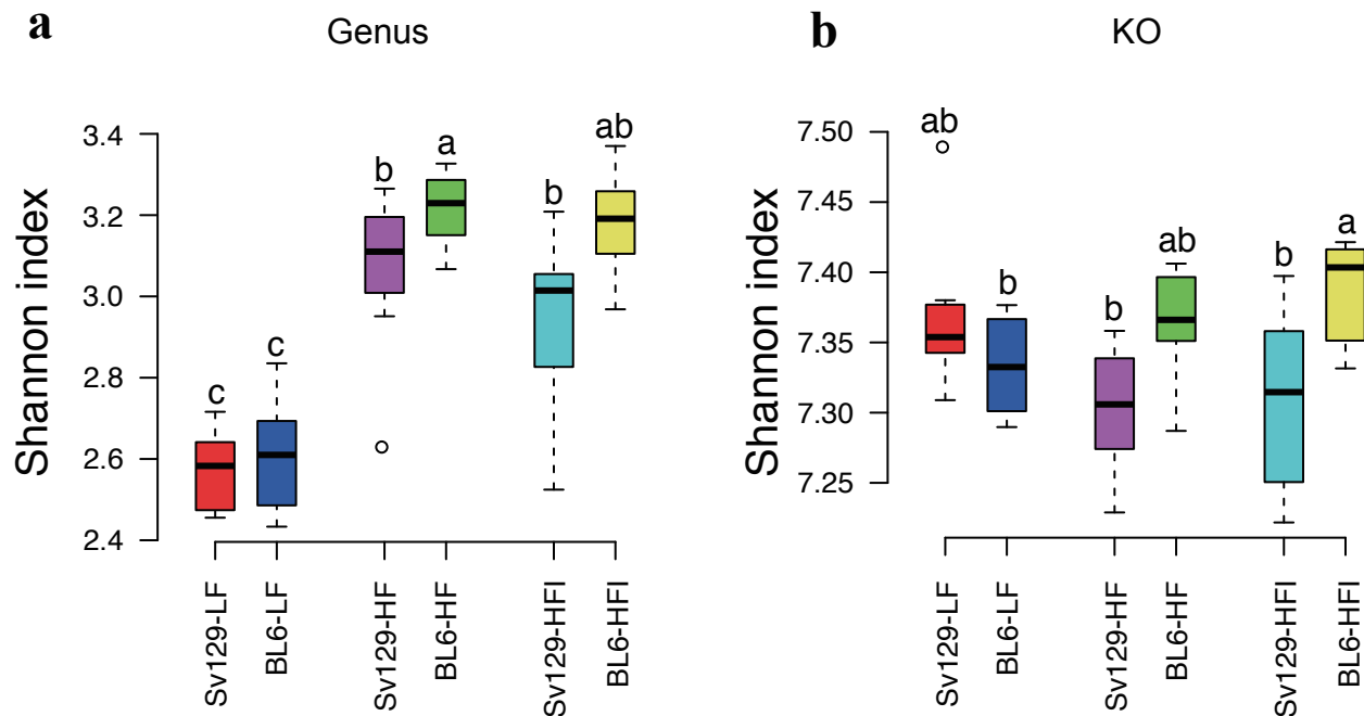
Figure S5. Alpha diversity based on (a) genus and (b) KO profiles. At the genus level, HF feeding increased alpha diversity in both Sv129 and BL6, while at the KO level HF feeding did not increase alpha diversity relative to LF feeding. Comparison between mouse strains showed that alpha diversity at the KO level in HF fed mice was higher in BL6 mice than in Sv129 mice. Statistic differences were analyzed by unpaired Wilcoxon Rank-Sum test (with FDR correction). Statistically significant differences ( P < 0.05 ) between groups are denoted with different letters (a, b, c, d) on the top of the graphic boxes.
