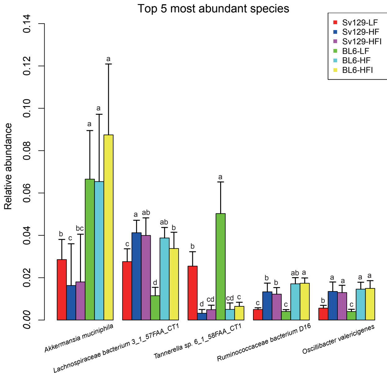
Figure S10. The top 5 most abundant annotated species in relation to mouse strain and diet. The figure shows the top 5 most abundant annotated species, which also clearly exhibited significant changes in abundance in relation to diet. Statistical differences were analyzed by unpaired Wilcoxon Rank-Sum test (with FDR correction). Statistically significant differences ( P < 0.05 ) between groups are denoted with different letters (a, b, c, d) on the top of the graphic boxes.
