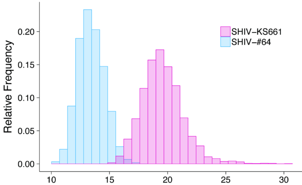
Figure S2 | Distribution of basic reproduction numbers without removal for SHIV-KS661 and -#64 in HSC-F cells. The distributions of the basic reproduction numbers without the effect of removal, R_0 = \beta_{50}p_{50}T(0)/\delta(c_{RNA} + c_{50}) , that were calculated from the estimated parameter distributions are shown for SHIV-KS661 (red) and -#64 (blue) strains. The basic reproduction number for SHIV-KS661 is significantly different from that for SHIV-#64, as assessed by the repeated bootstrap t -test.
