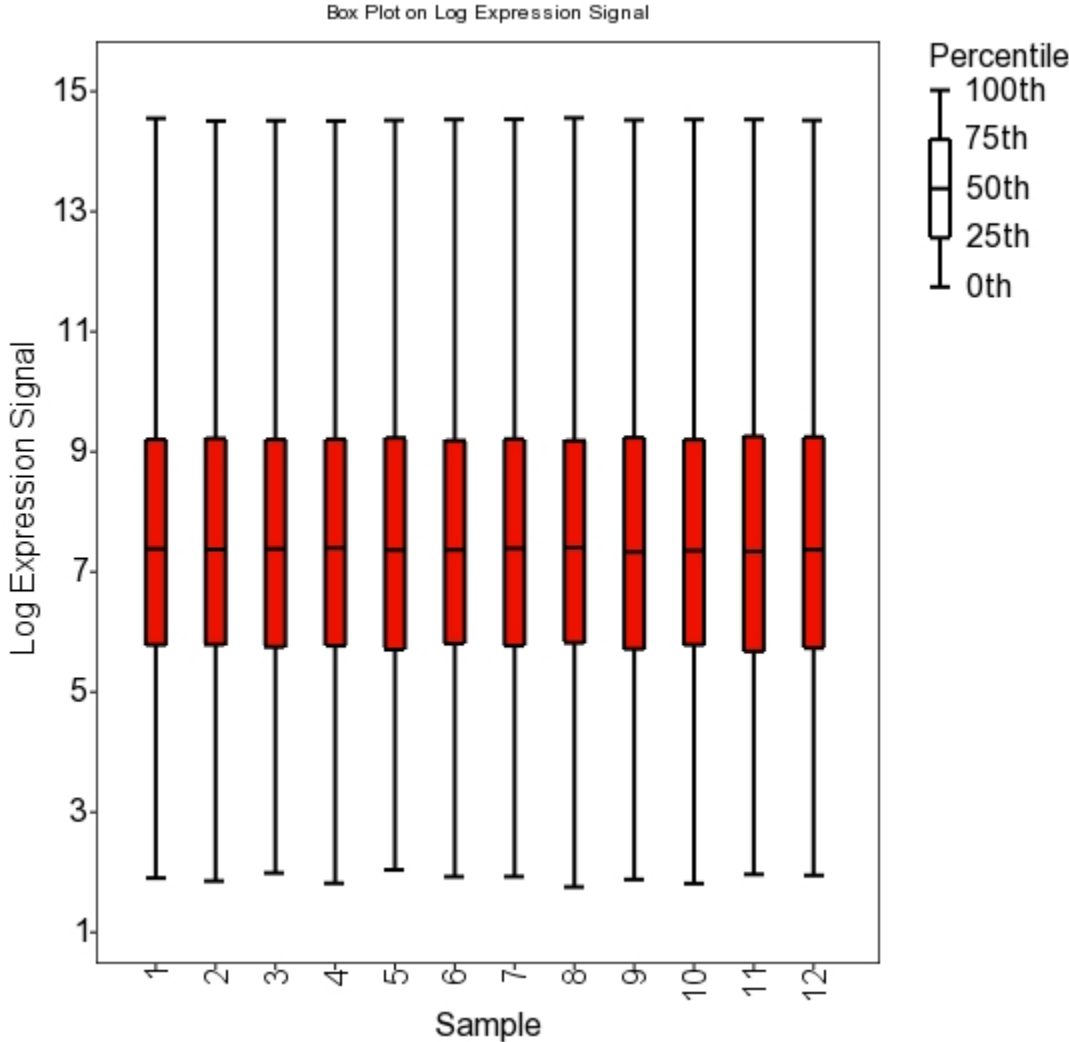
Supplementary Figure 1. Box plot of the \log_2 expression signal for each sample (microarray chip).
