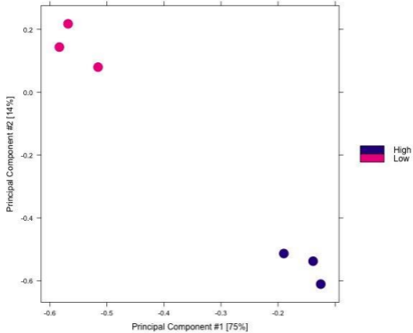
PCA: Condition
