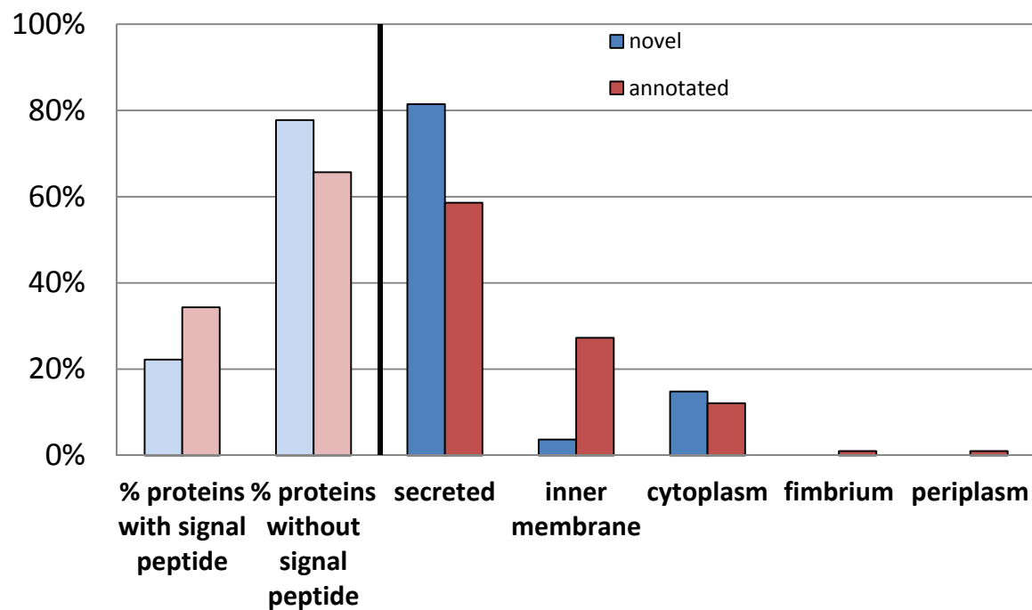
(Left part) Graphical overview of novel and length-matched annotated proteins either possessing a signal peptide detected using SignalP or not. (Right part) Predicted subcellular localization using LocTree3. Note, that for the analysis shown here only proteins with one predicted transmembrane-domain (TMD) were considered.
