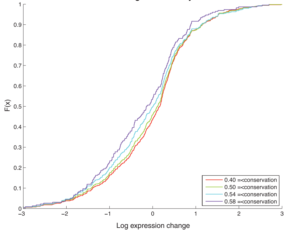
CDF of miR-15a targets filtered by conservation
