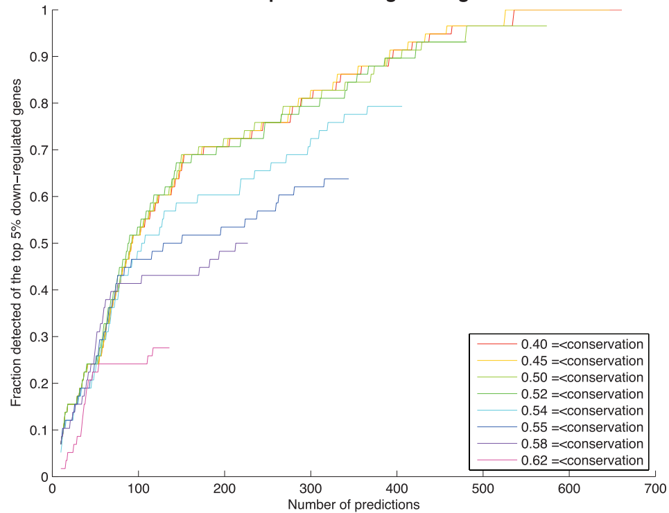
Detection of miR-15a canonical targets in the top 5% down-regulated genes
