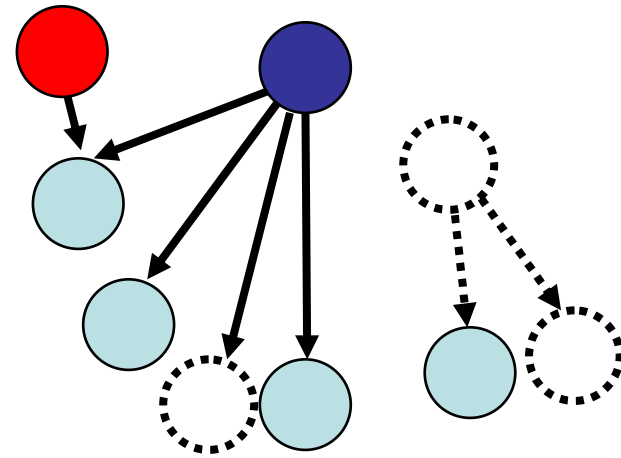
Changes in the repertoire of TFs and targets in organism B
