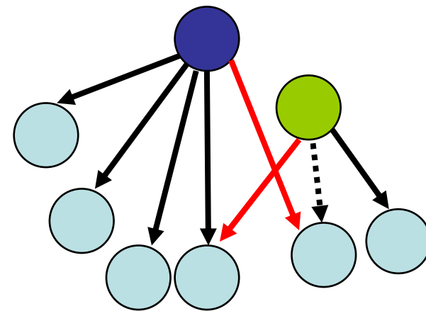
Rewiring the interactions within the TRN of organism B
