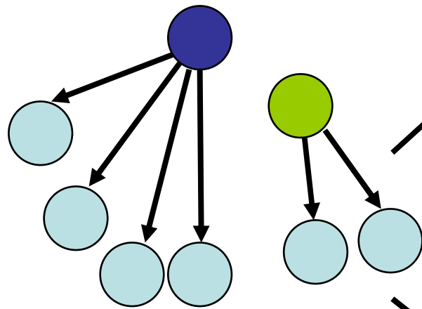
TRN organism A
