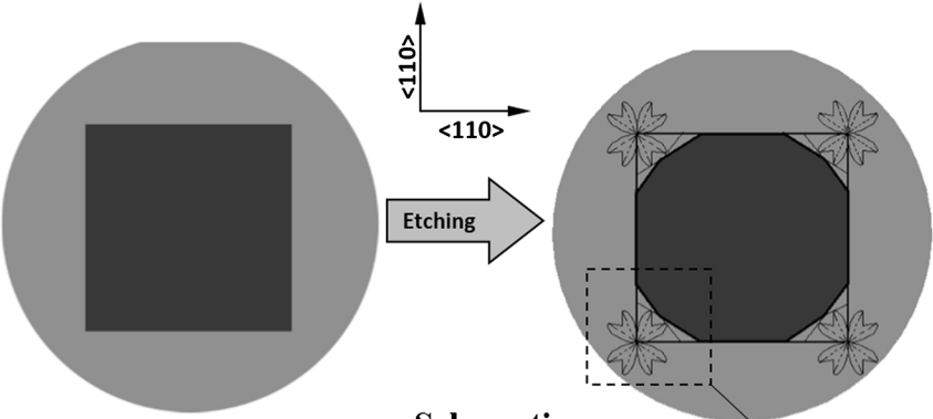
A masked pattern on \{100\} wafer
