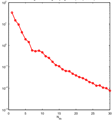
Convergence of the greedy algorithm (dual problem)
