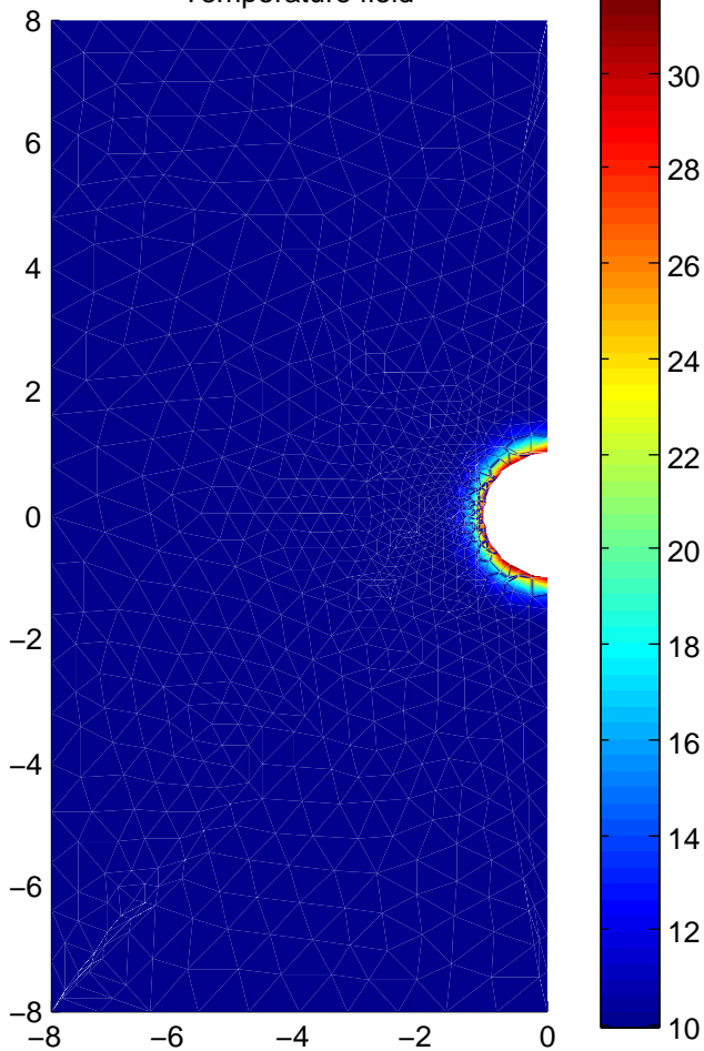
Temperature field
