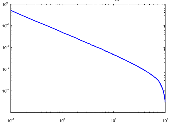
Lower bound coercivity constant \alpha_{LB}(\mu)
