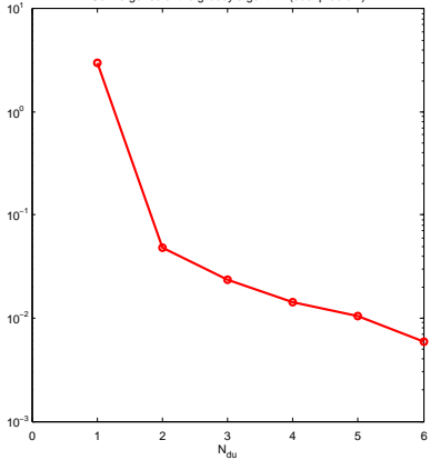
Convergence of the greedy algorithm (dual problem)
