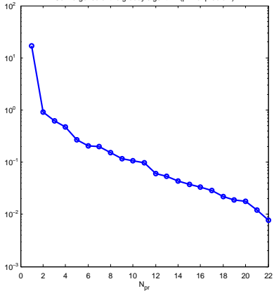
Convergence of the greedy algorithm (primal problem)
