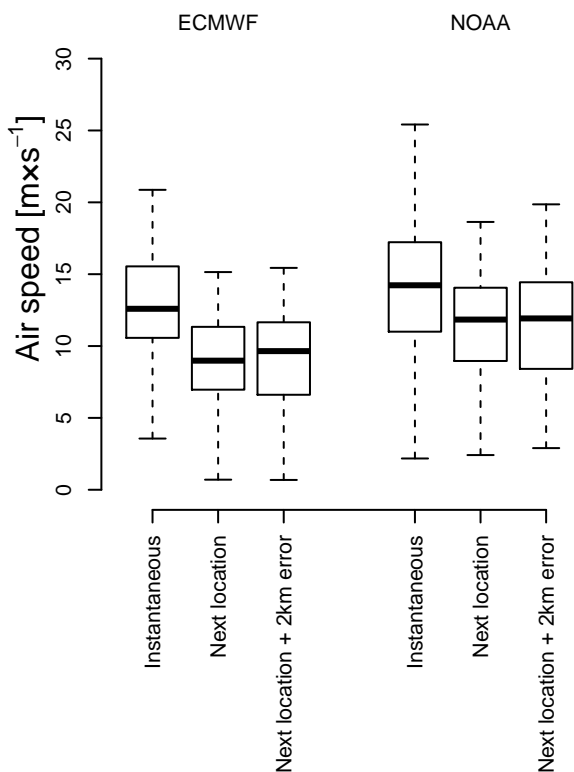
Larus scoresbii
