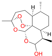
dihydroartemisinin (9)
