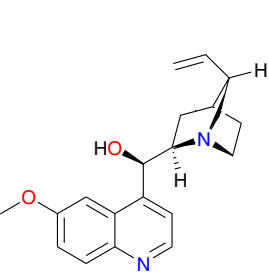
quinine (3)
