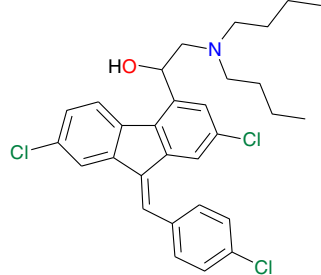
lumefantrine (6)
