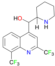
mefloquine (4)
