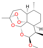
artemether (10)
