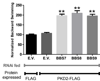
C. PKD2-FLAG : 25 mM TEA / 10 mM NaCl
