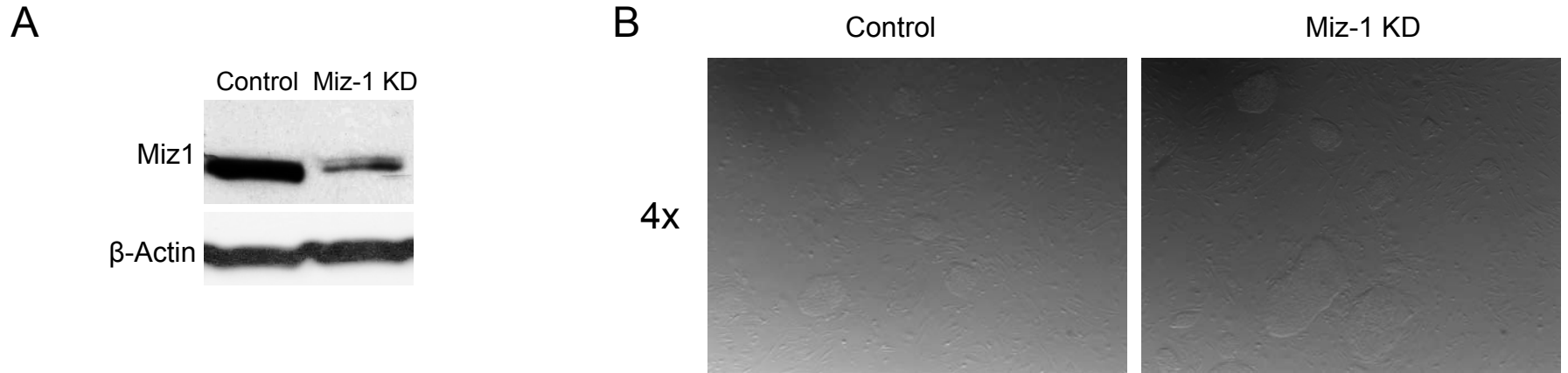
Figure S3. Confirmation of Miz-1 KD in human ES cell. A. Western blot analysis of Miz-1 protein levels. B. Phase contrast images of human ES cells transduced with either scrambled shRNA control or shRNA specific to Miz-1. Images were taken at 4x magnification.
