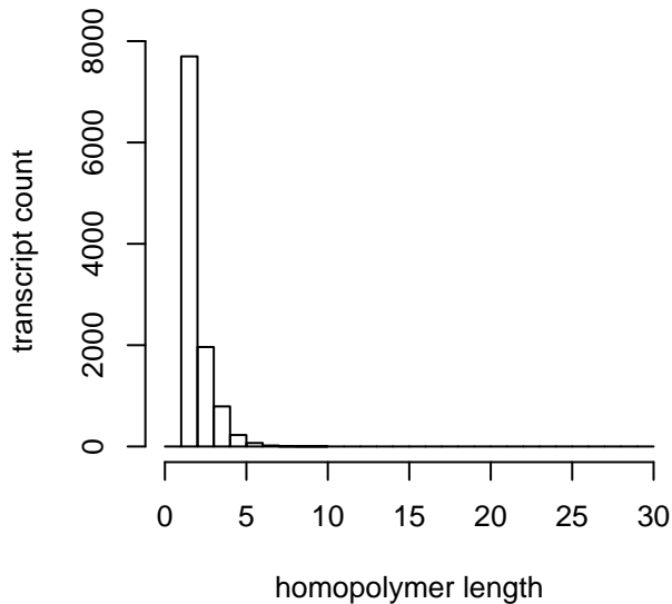
A homopolymer length distribution
