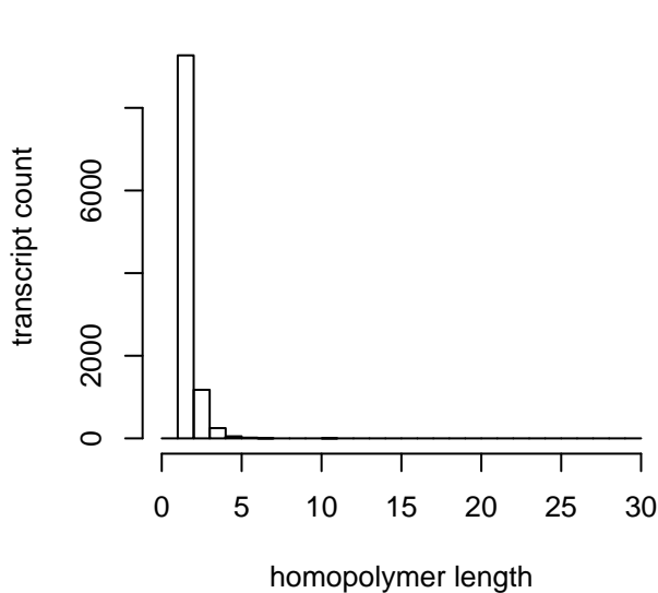
C homopolymer length distribution
