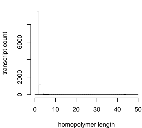
G homopolymer length distribution
