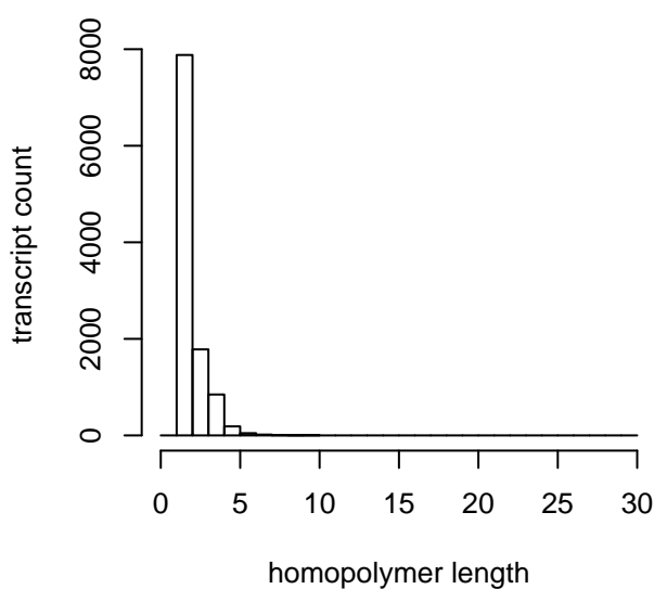
T homopolymer length distribution
