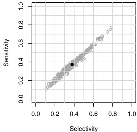
16S Prediction Accuracy UNAFold
