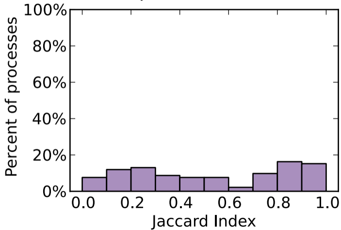
A Genes-based overlap of processes
