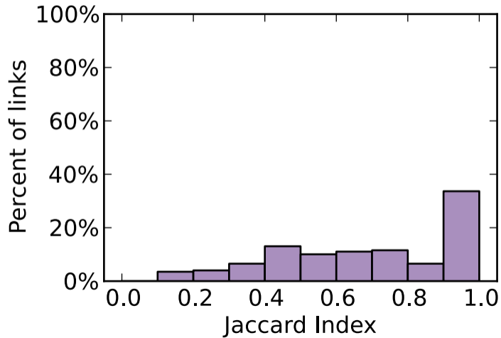
B Overlap between links based on cross-annotated interactions
