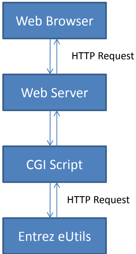
Standard use of Entrez eUtils by a Web Application
