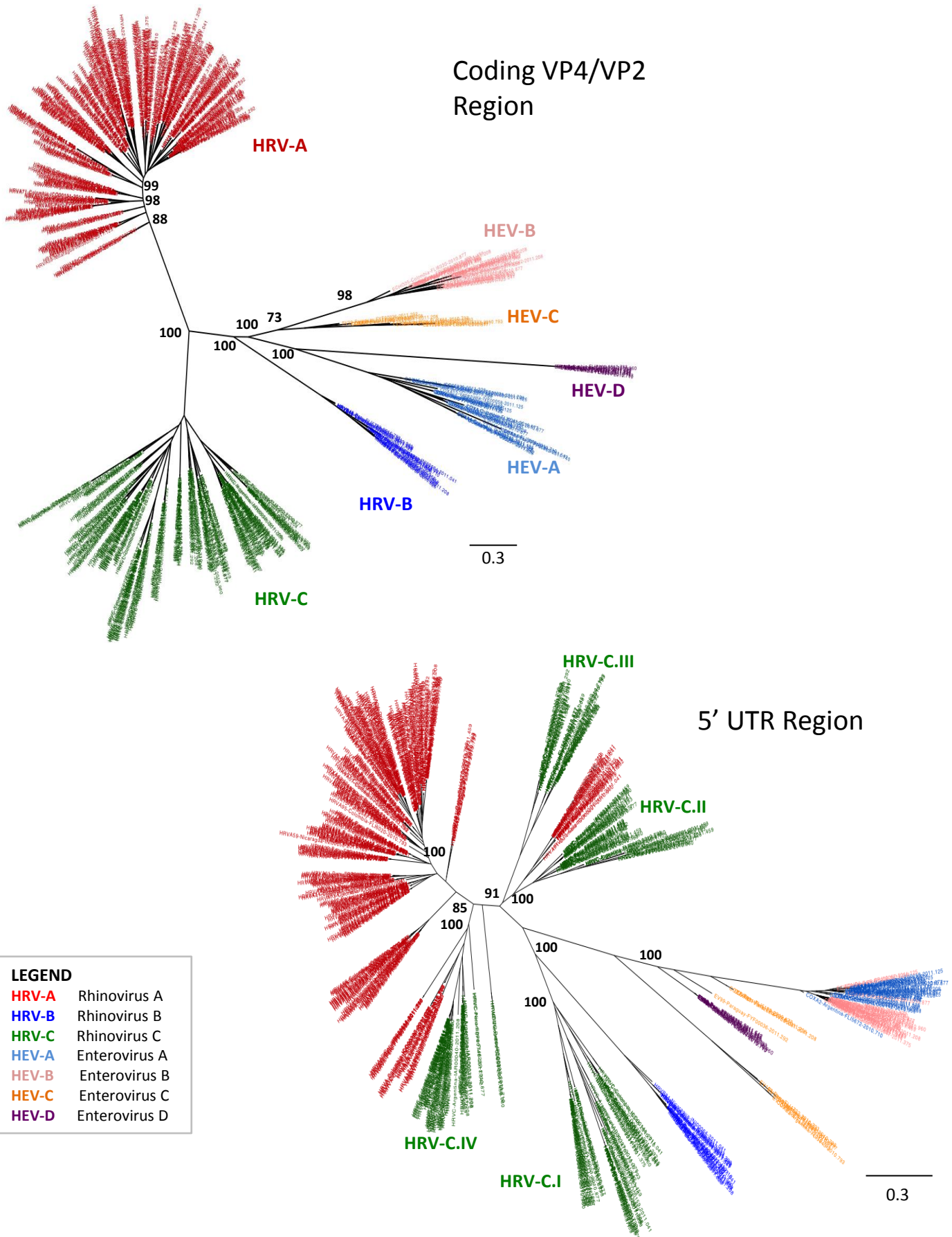
Figure 6: Phylogenetic analyses of HRV and HEV
