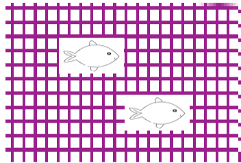
phishGILLNET
