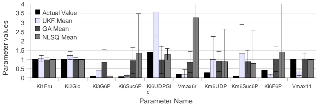
Comparison of parameter estimation methods
