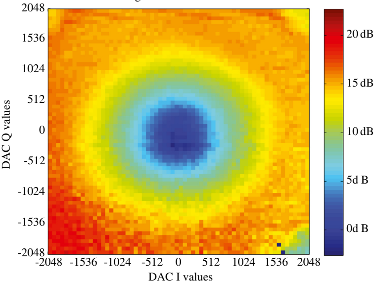
Fast Algorithm Isolation Gain
