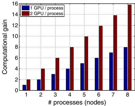
(b) Multi-node GPU cluster
