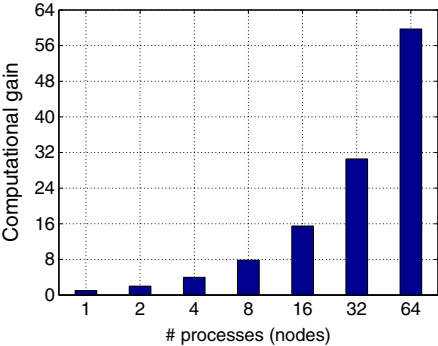
(a) Multi-node CPU cluster
