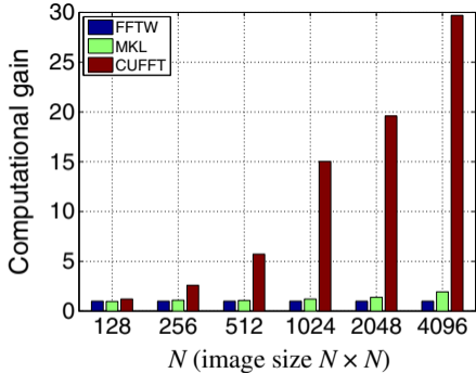
(b) Double-precision data
