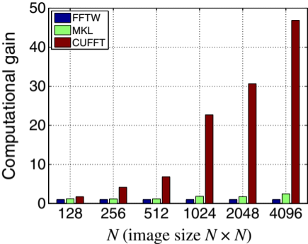
(a) Single-precision data
