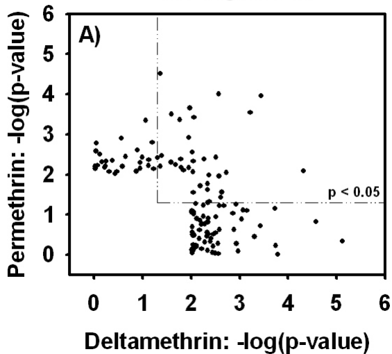
PIR Regression
