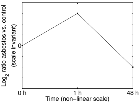
Met5A cell line, model profile of cluster 3
