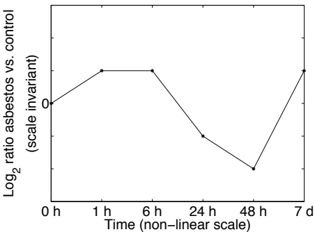
A549 cell line, model profile of cluster 9
