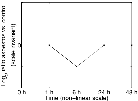
BEAS-2B cell line, model profile of cluster 8
