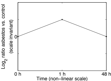
Met5A cell line, model profile of cluster 1
