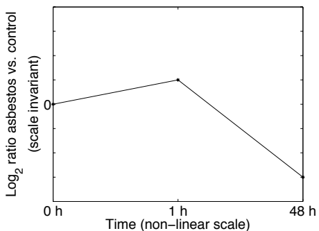
Met5A cell line, model profile of cluster 2
