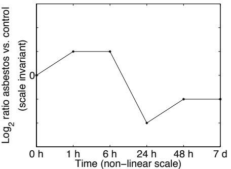
A549 cell line, model profile of cluster 5
