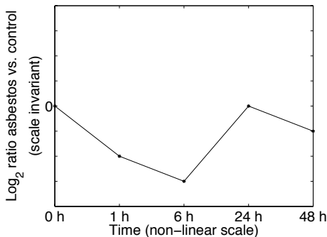
BEAS-2B cell line, model profile of cluster 5
