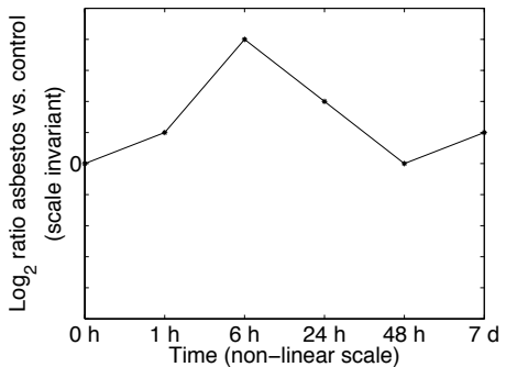
A549 cell line, model profile of cluster 1
