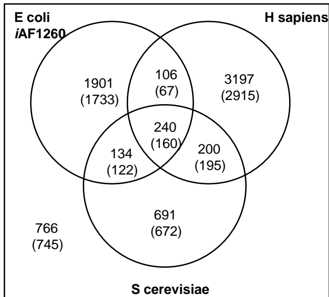
a) Reactions
