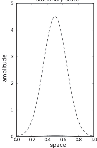
stationary state
