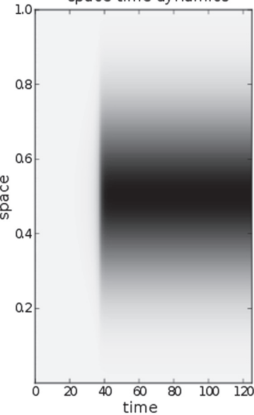
space-time dynamics
