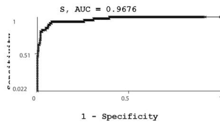
ROC plot for PSM module
