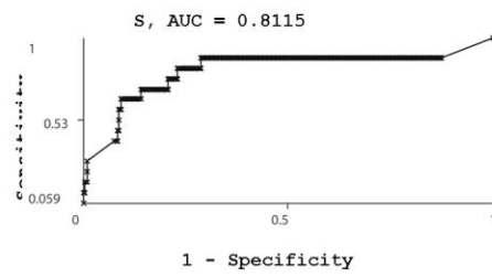
ROC plot for CPF module
