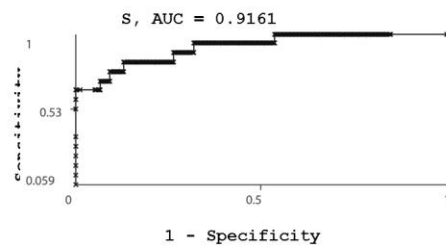
ROC plot for CTD module
