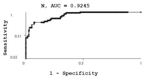
ROC plot for CTD module
