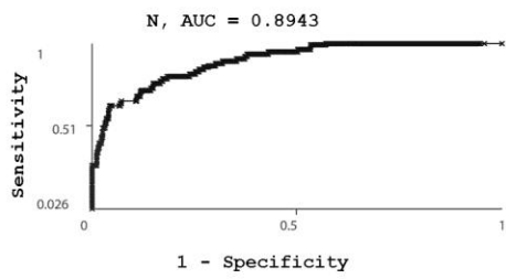
ROC plot for PSM module
