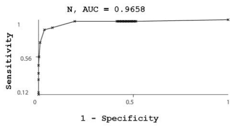
ROC plot for HYB module
